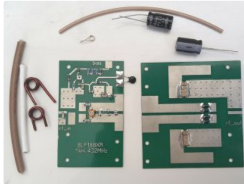
500W-1KW 432MHz LDMOS Power Amplifier kit
